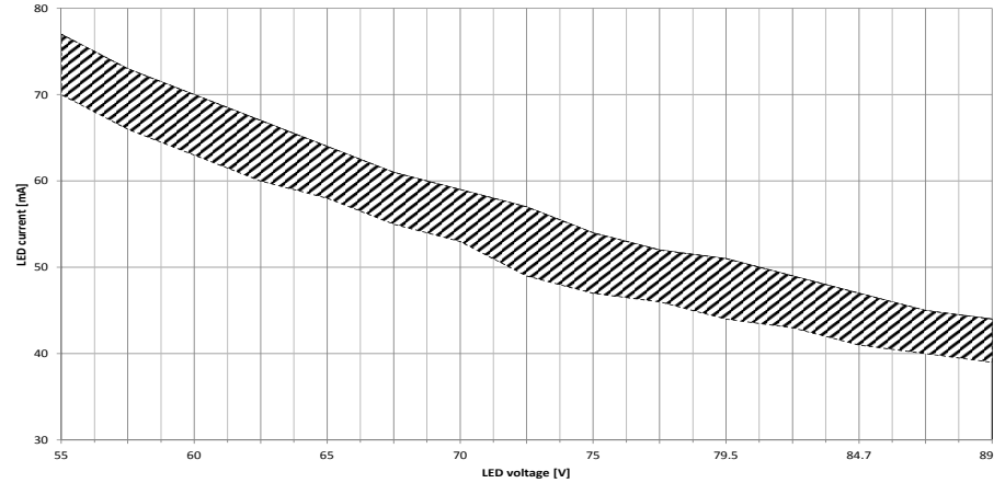
3.5W - OL90/4/DST
